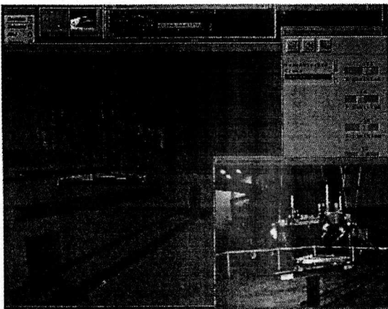
Fig. 1: 3-D visualization of a robotic crane during an assembly operation with a steel I-beam. The inset video image shows the correspondence between the model and the real system. The real-time data driving the visualization subsystem came from TETRA's real-time controller, via the tetSock proto-protocol.
