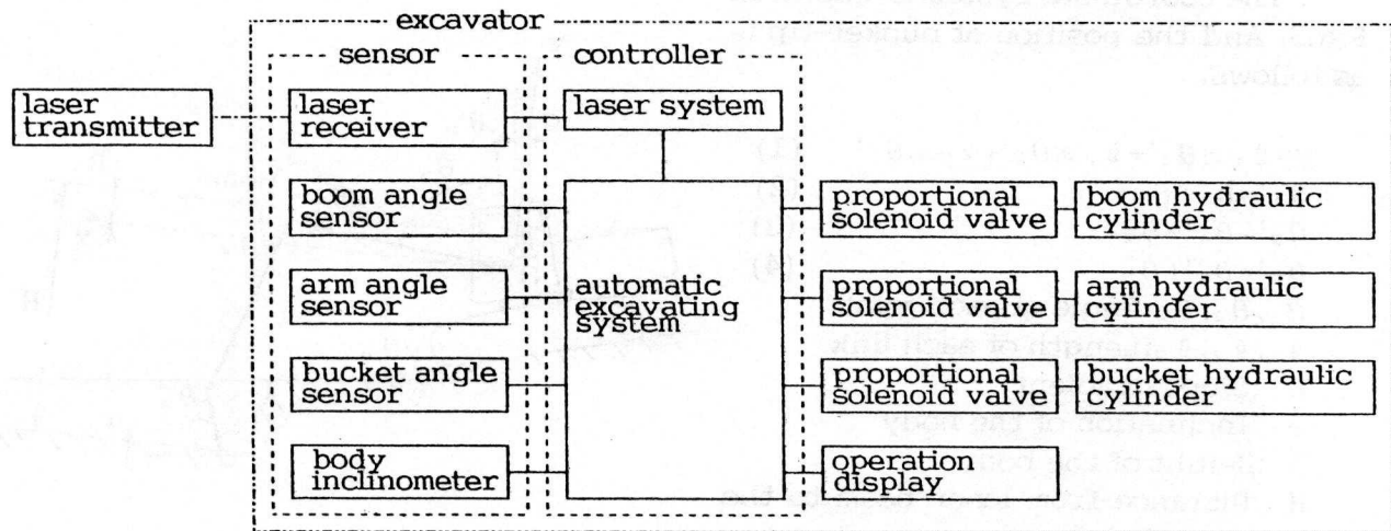
Fig.2 System Scheme
