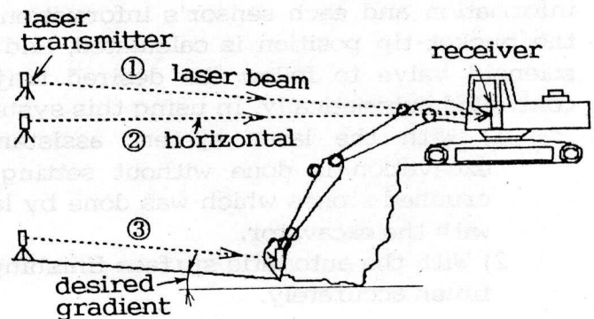
Fig.5 Laser Position
