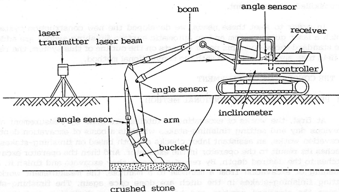
Fig.1 Automatic Excavation System
