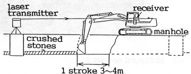
b) Excavating and Finishing
