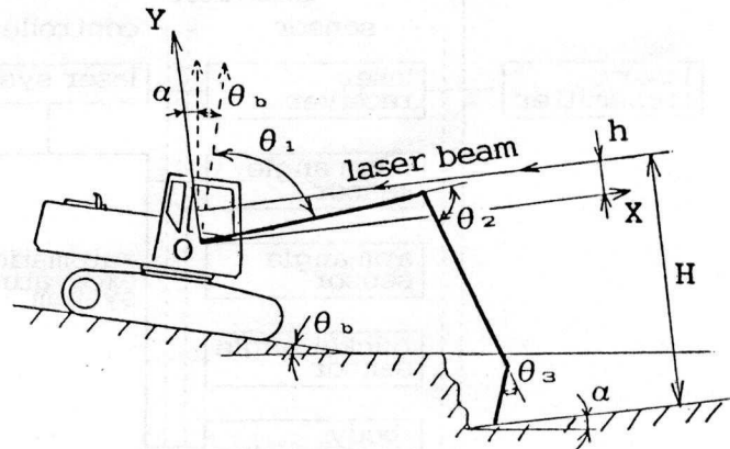
Fig.3 Coordinate System
