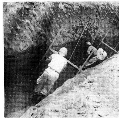
Fig. 8 Comparison between New Method and Conventional Method
